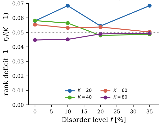
(b) Rank deficit vs disorder (selected K )
