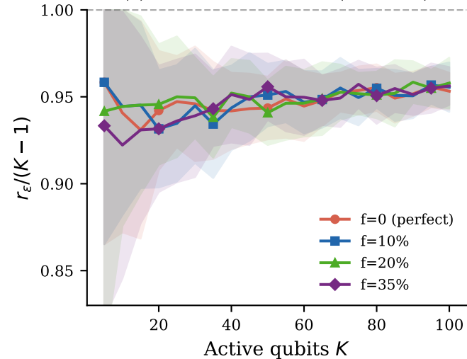
(a) Disorder robustness ( \nu = 20a/T )
