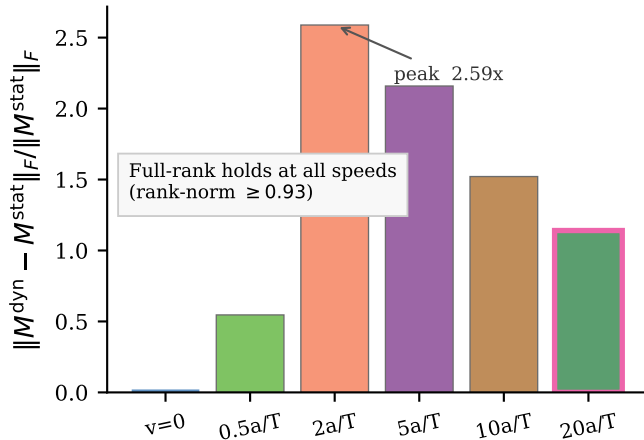
(b) Matrix deviation from static limit ( K = 20 , 12 realisations)
