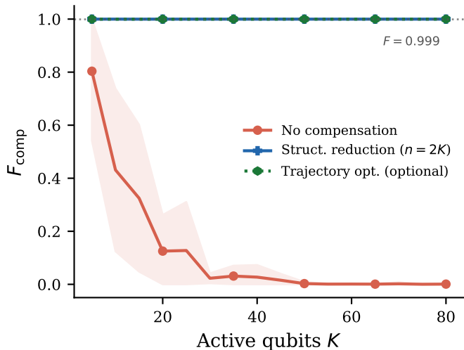
(a) F_{\text{comp}} vs active qubits K (random routing, u_j \sim \mathcal{U}[-U_j, U_j] )
