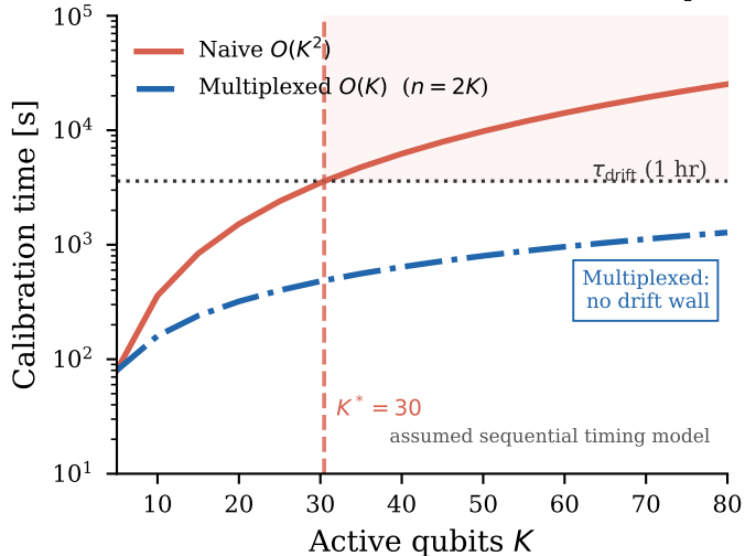
(b) Calibration cost: O(K^2) naive vs O(K) multiplexed
