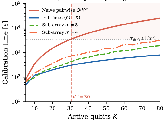
(a) Calibration time vs K (sub-array multiplexing)
