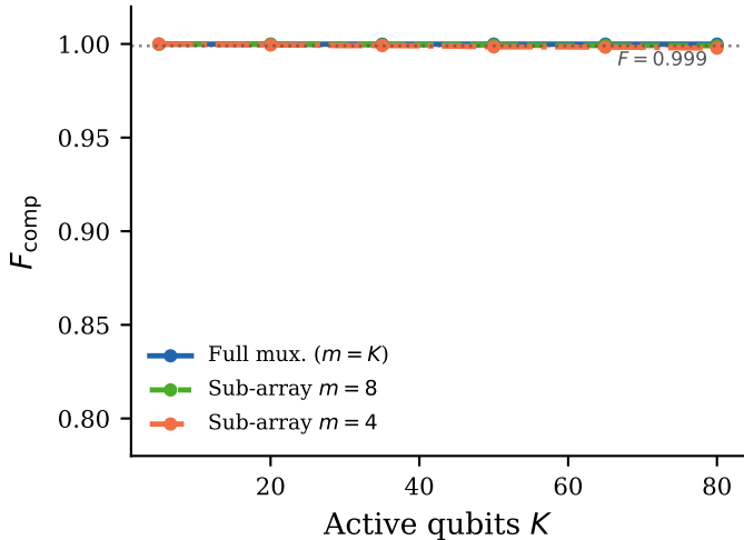
(b) F_{\text{comp}} at n_{\text{exp}} = 3K rounds (finite-channel multiplexing)
