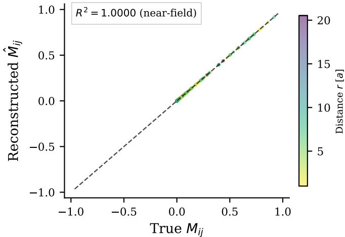
(a) Structural reduction: reconstruction accuracy ( n_{\text{exp}} = 2K , 1/r^3 prior, K = 40 )
