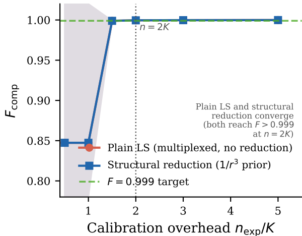
(b) F_{\text{comp}} vs calibration overhead ( K = 40 )
