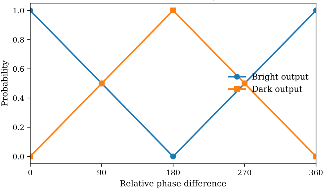
Phase difference moves probability between outputs
