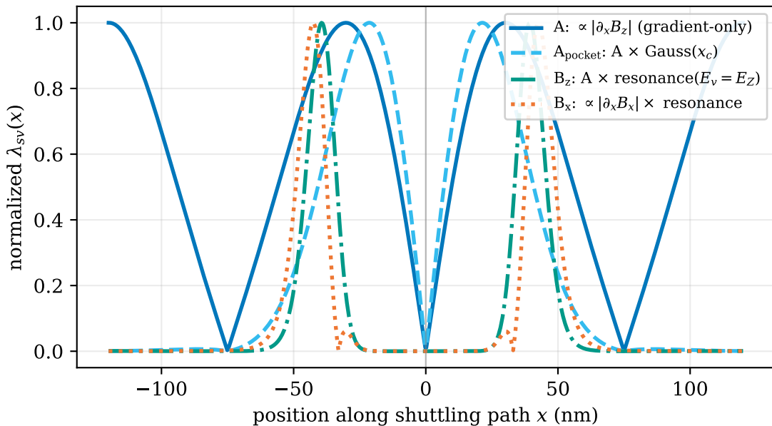
Four phenomenological coupling ansatz \lambda_{sv}(x)
