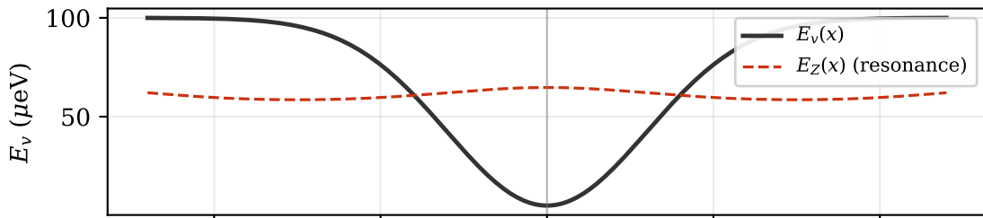
Valley splitting profile and spin--valley resonance
