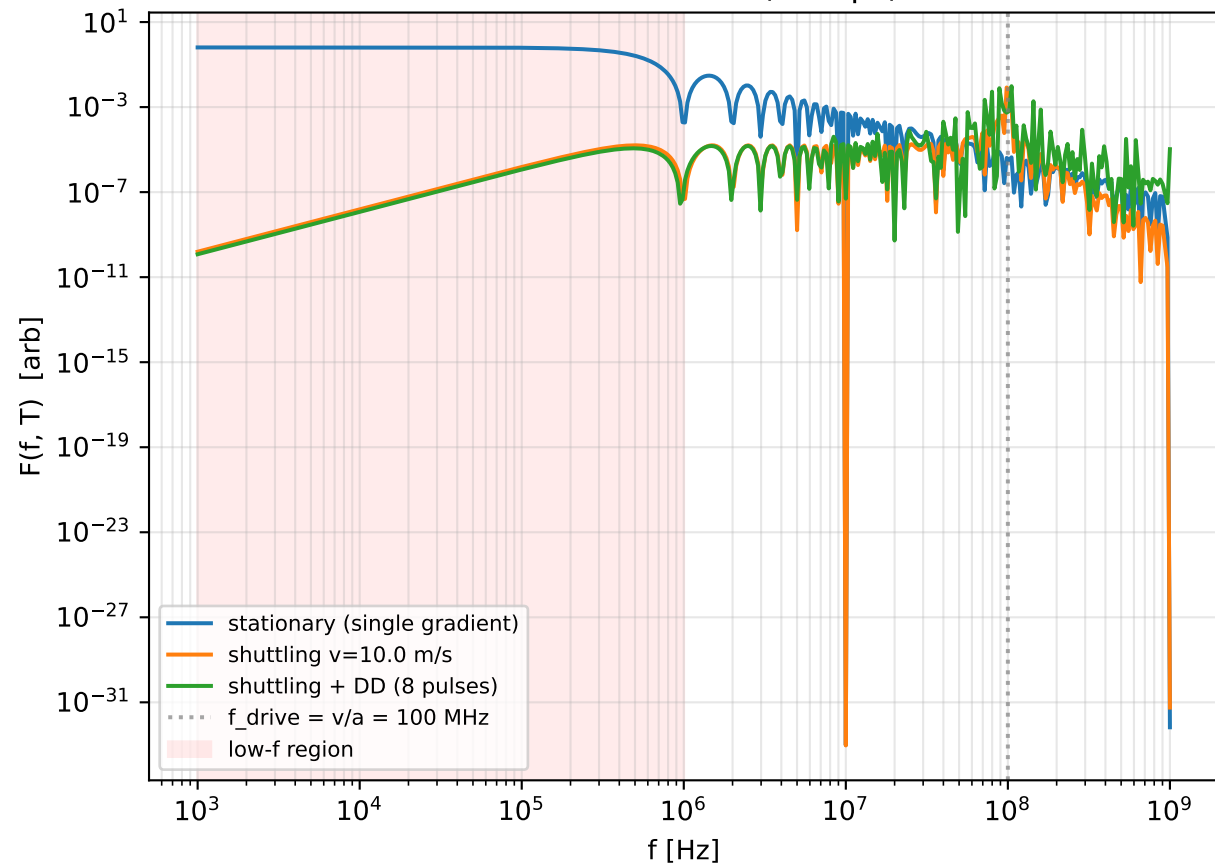
B3: Filter function ( T=1\text{ }\mu\text{s} )
