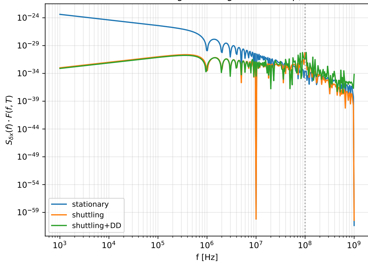
B3b: PSD-weighted integrand (overlap)
