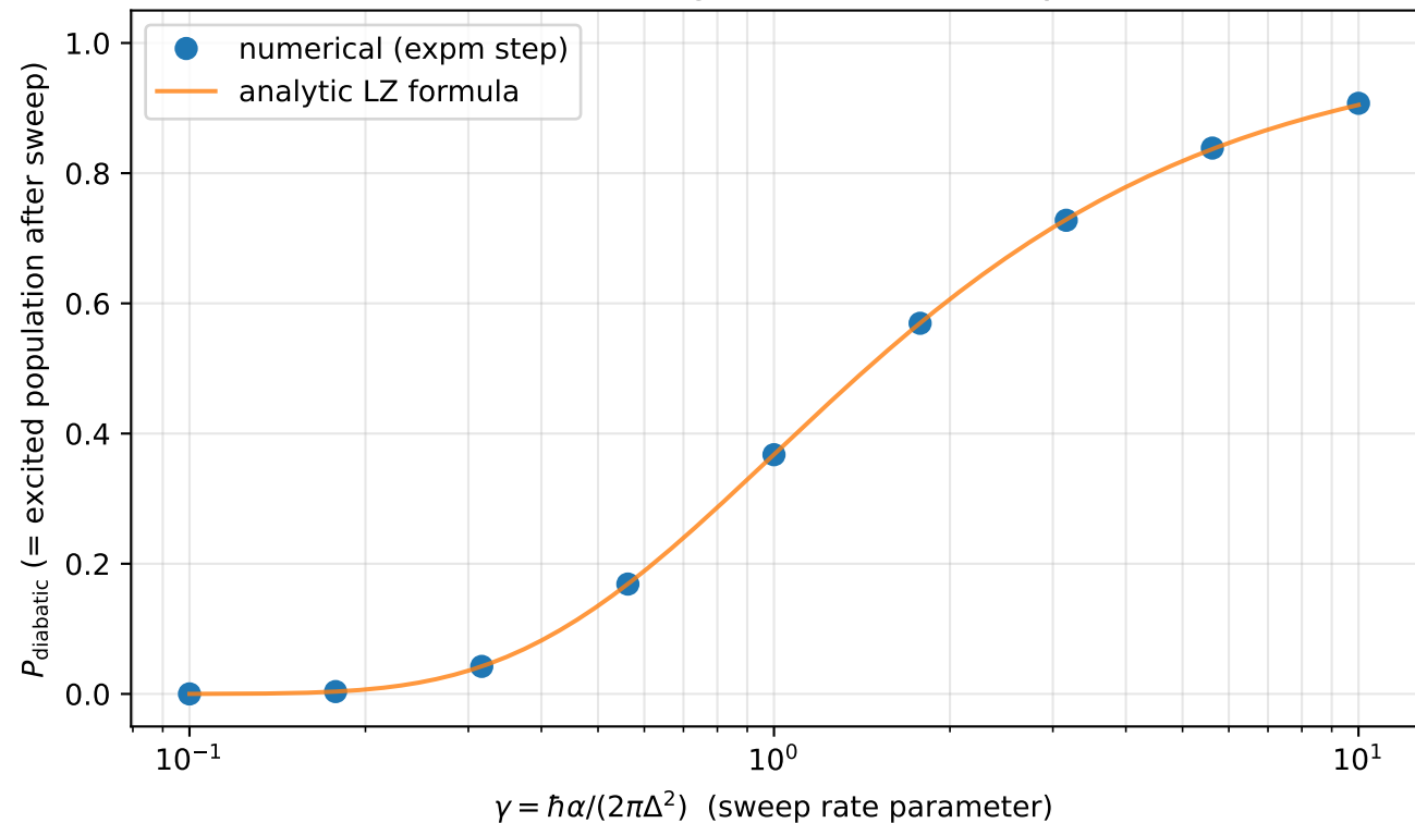
C1: LZ crossing, numerical vs analytic
