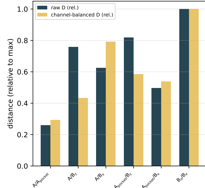
(3) Model distance ( B_z vs B_x largest; ranking reorders)
