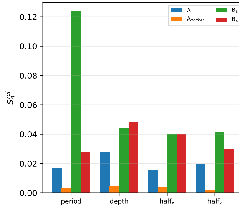
(4b) Relative geometry sensitivity (no shared hierarchy; B_z : period largest)
