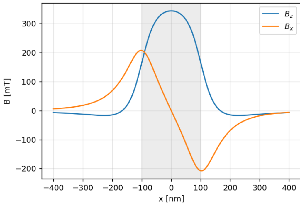
z = -100 \text{ nm} (2DEG) — field
