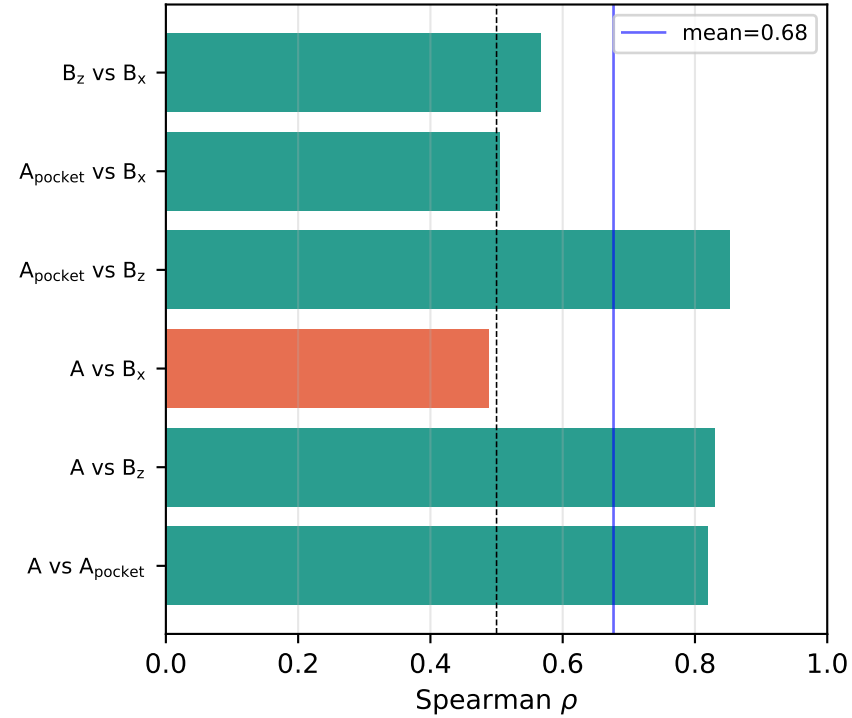
(1) Rank correlation (partial ansatz-dependence)
