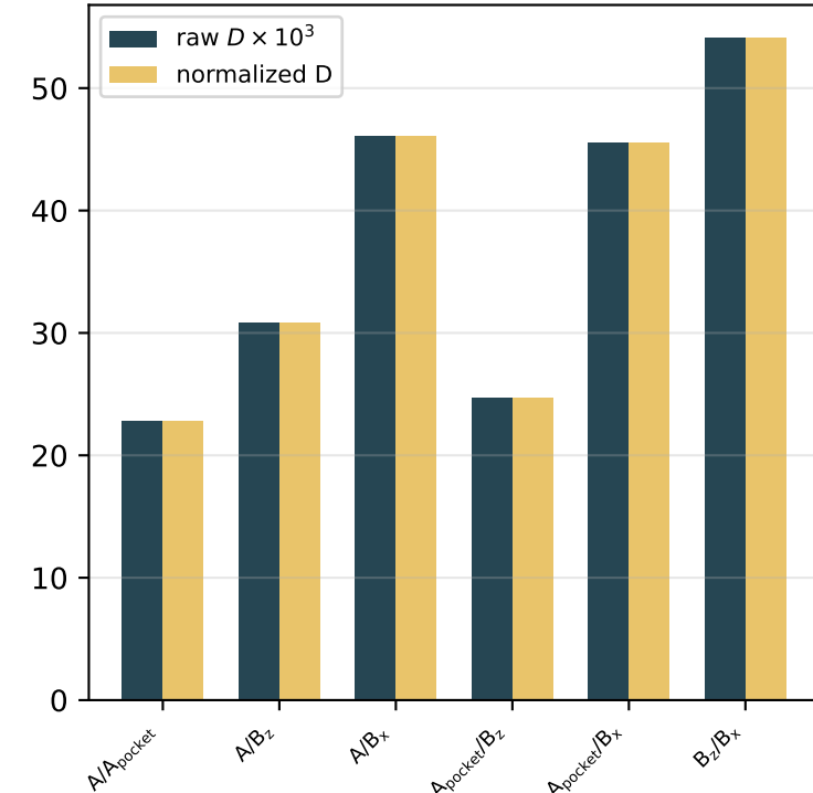
(3) Model distance ( B_z vs B_x largest)
