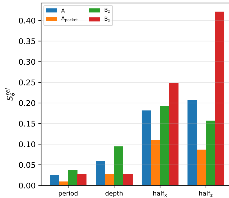
(4b) Relative geometry sensitivity (hierarchy weakened; period smallest)
