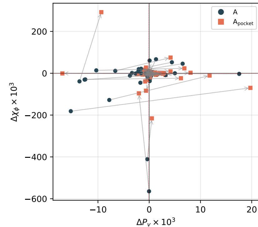
(5) A \rightarrow A_{\text{pocket}} quadrant shift (71 disagreement conditions)
