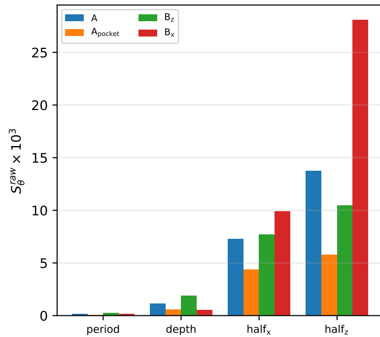
(4a) Raw geometry sensitivity ( \text{half}_z dominant)
