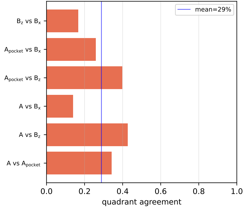
(2) Quadrant agreement (stronger ansatz-dependence)
