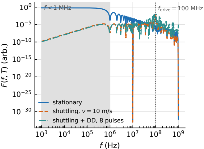
(a) filter function, T = 1 \mu\text{s}
