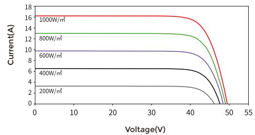
Current-Voltage Curve
