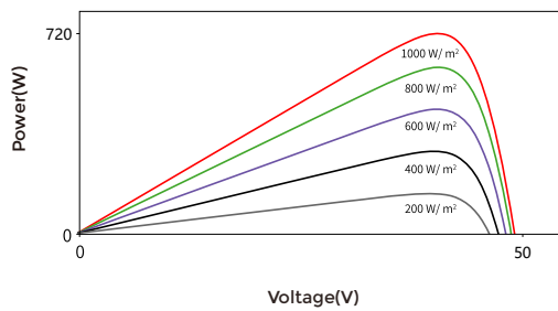
Power-Voltage Curve
