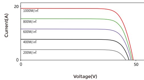
Current-Voltage Curve
