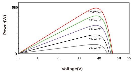
Power-Voltage Curve
