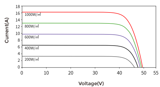
Current-Voltage Curve
