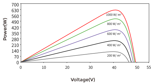
Power-Voltage Curve
