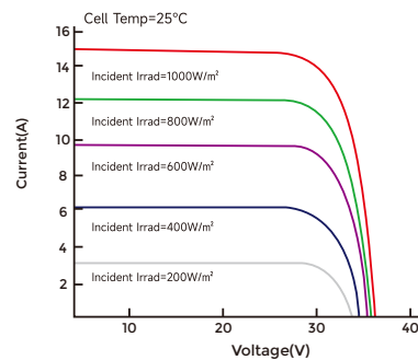
Current-Voltage Curve
