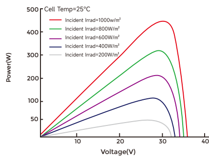
Power-Voltage Curve
