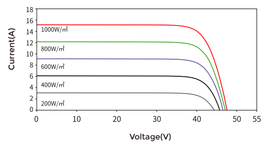
Current-Voltage Curve
