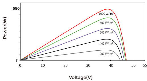
Power-Voltage Curve
