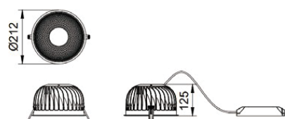
D200 Opening range Ø125–130mm
