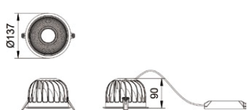
D125 Cut-out range Ø125–130mm
