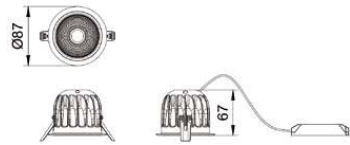
D75 Cut-out range Ø75–80mm
