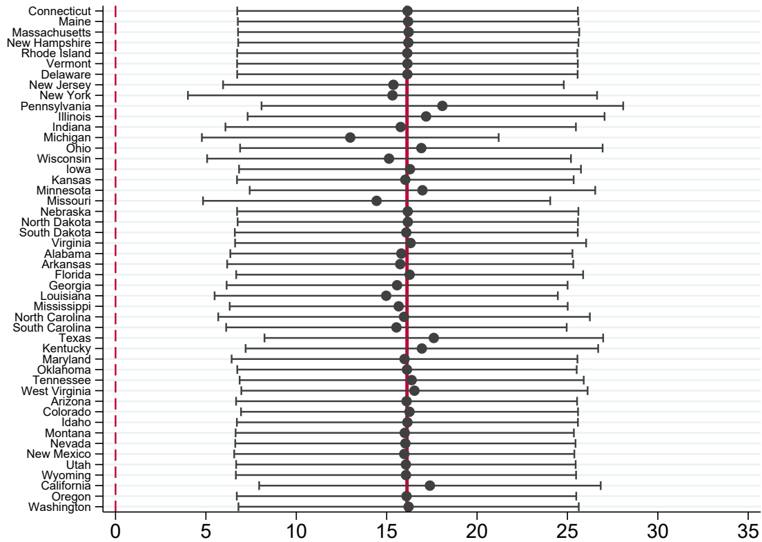
Figure A.9: Leave one state out estimator
