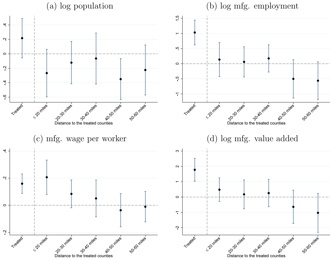
Fig. 5. Spatial spillover.
