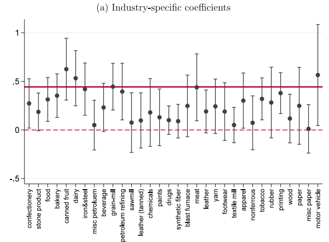
Fig. 8. Industry-specific estimates.
