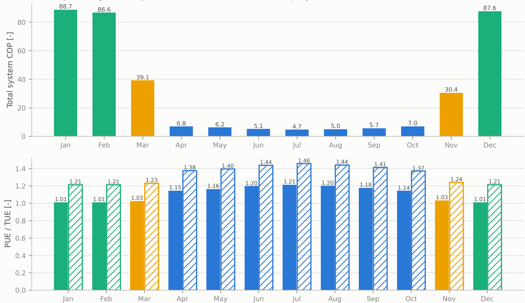
Monthly-average total system COP, PUE and TUE (Champaign, IL TMY3)
