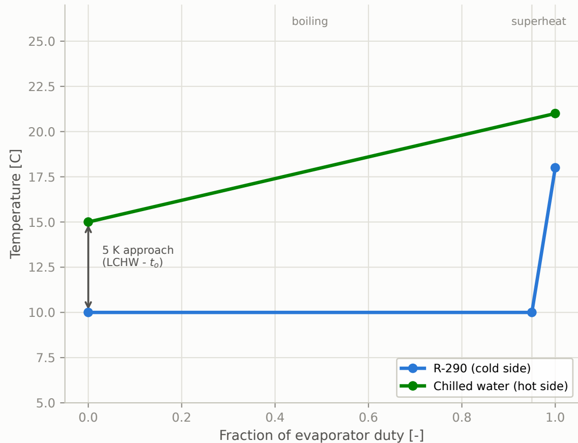
Evaporator --- two-zone profile (150 kW)
