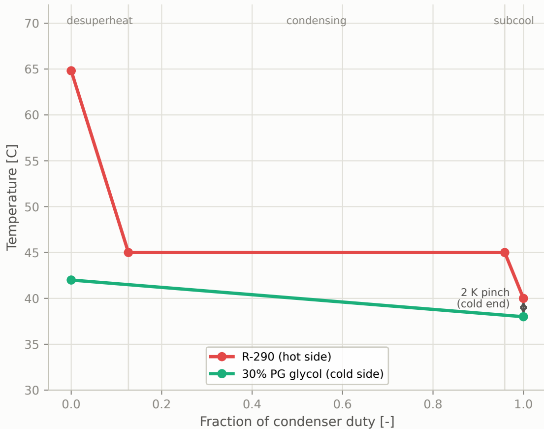
Condenser --- three-zone profile (181.7 kW)
