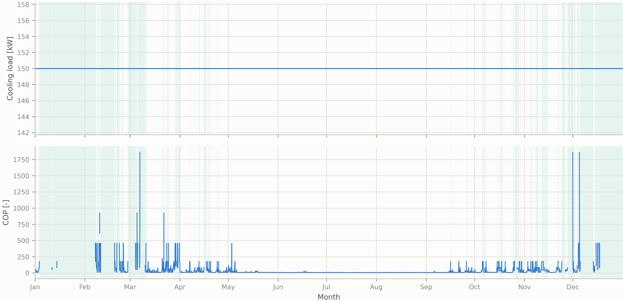
Delivered cooling load and compressor COP across the year (Champaign, IL TMY3)
