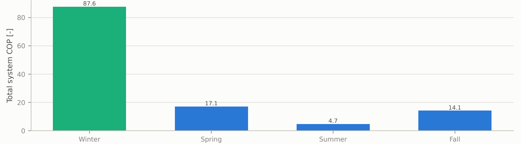
Seasonal-average total system COP, PUE and TUE (Champaign, IL TMY3)
