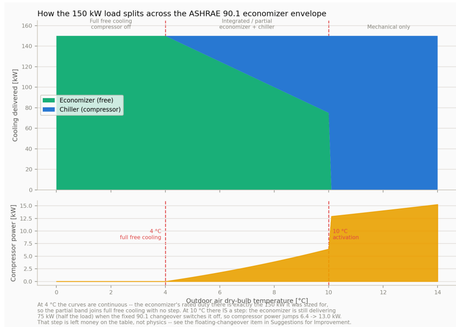
Load split & compressor power across the ASHRAE 90.1 economizer envelope
