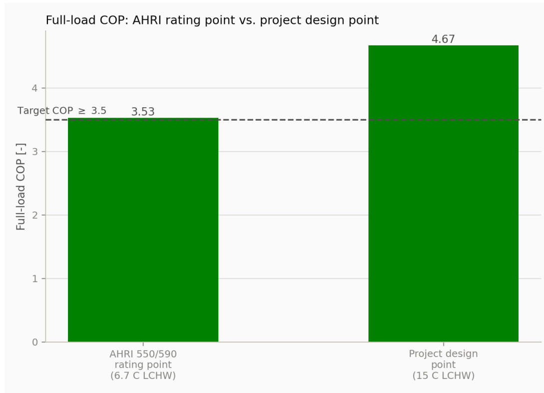
Full-load COP at the AHRI and project design points vs. the 3.5 target
