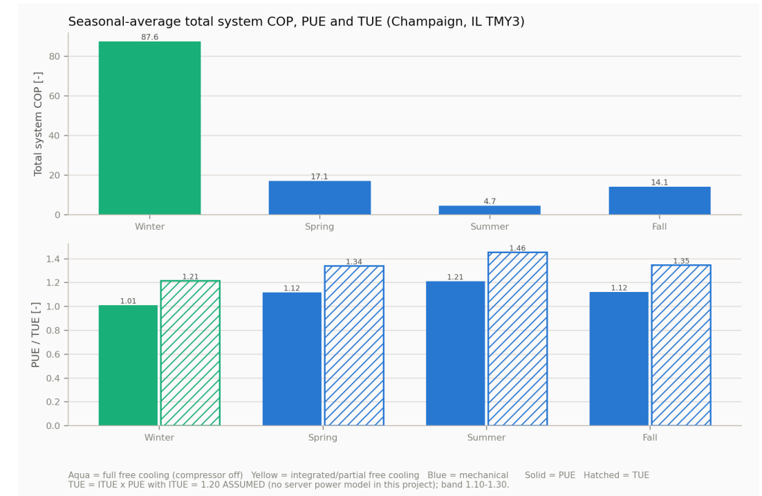
Seasonal-average total-system COP, PUE and TUE
