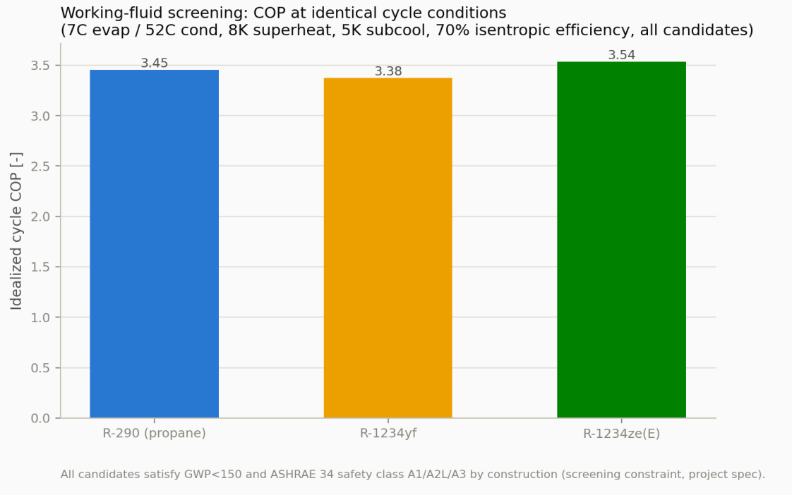
Cycle COP across screened refrigerant candidates
