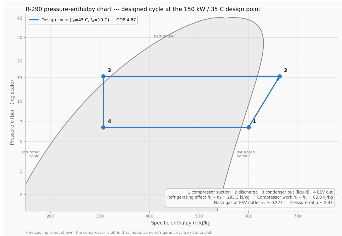
The designed cycle — R-290 p-h chart at 150 kW / 35 °C
