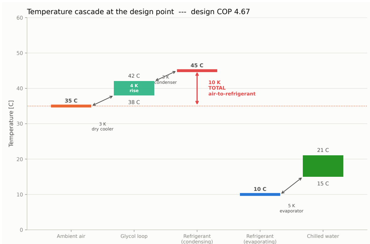
Figure 15.2. Temperature cascade from ambient air to chilled water at the design point. The condensing temperature is set by three approaches stacked in series.
