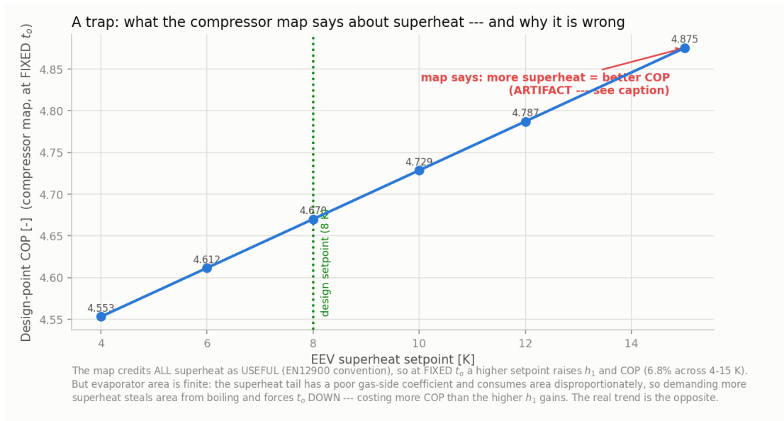
Figure 18.2. What the compressor map says about the superheat setpoint at fixed t_o — and why the trend is an artifact rather than a design lever.
