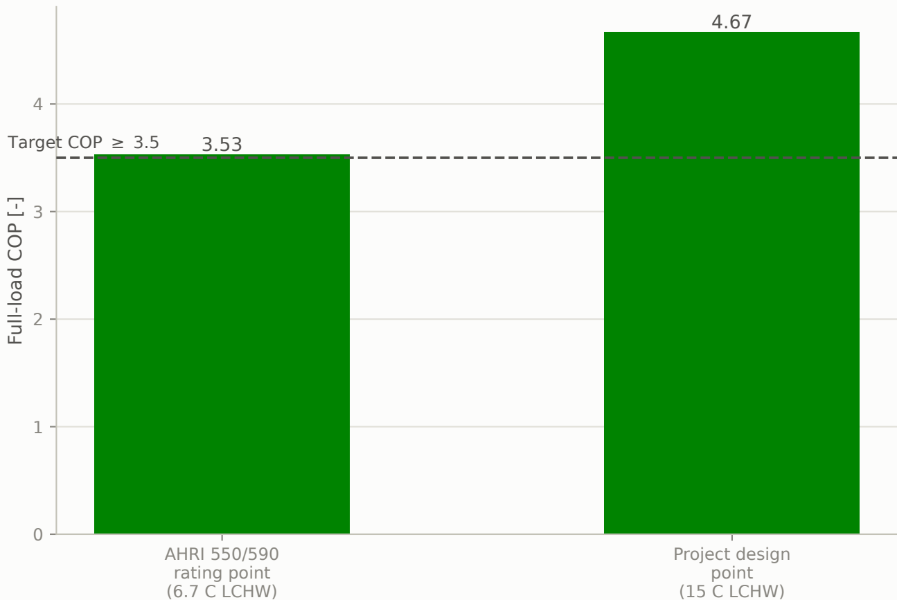
Full-load COP: AHRI rating point vs. project design point
