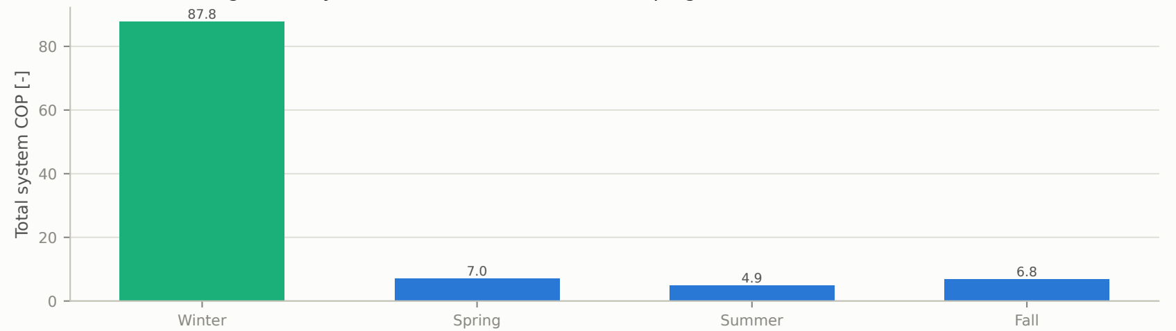
Seasonal-average total system COP, PUE and TUE (Champaign, IL TMY3)
