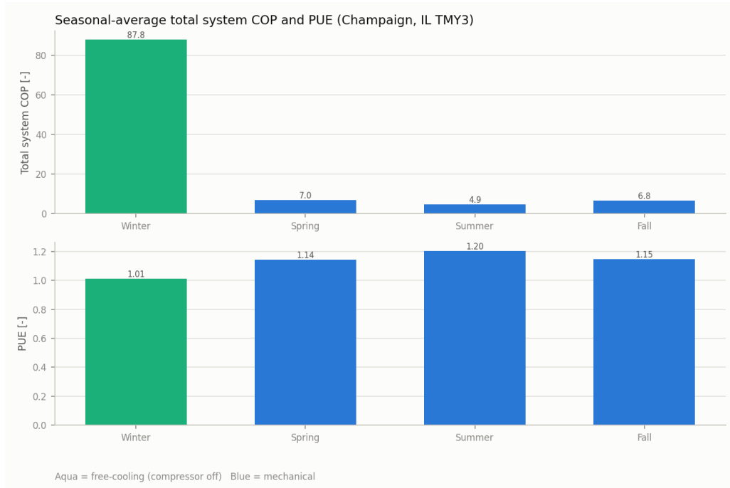
Figure 14.7. Seasonal-average total-system COP and PUE.
