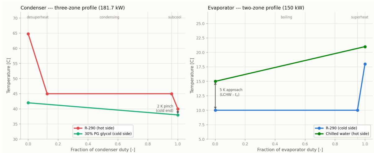
Figure 15.3. Counter-flow temperature profiles at the revised design point: condenser (three-zone) and evaporator (two-zone).
