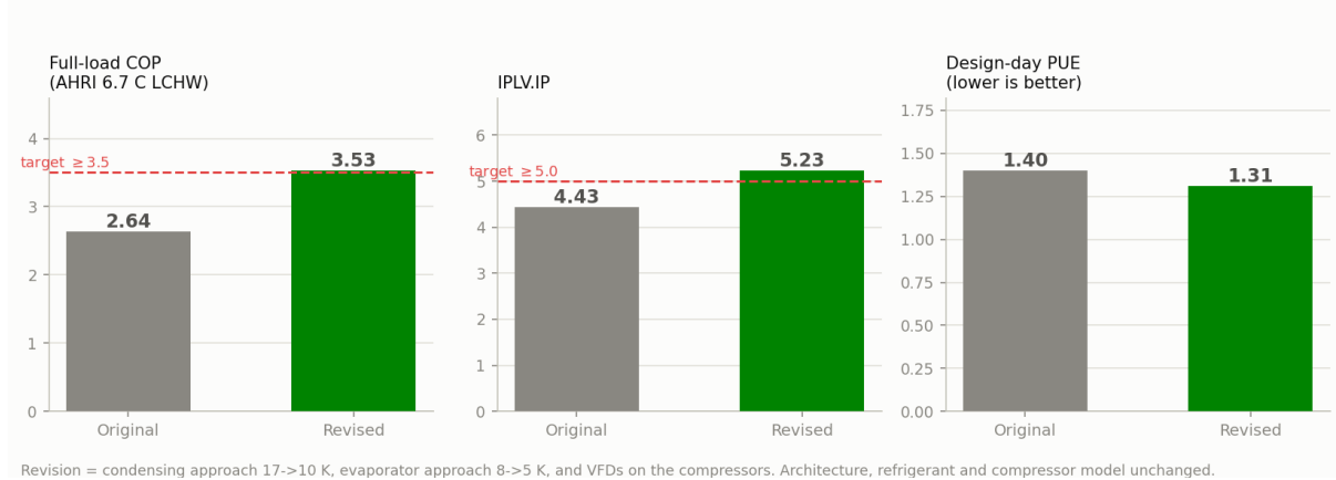
Figure 14.9. The revision’s headline result: both required metrics move from failing to compliant, and the design-day PUE improves as a by-product.
