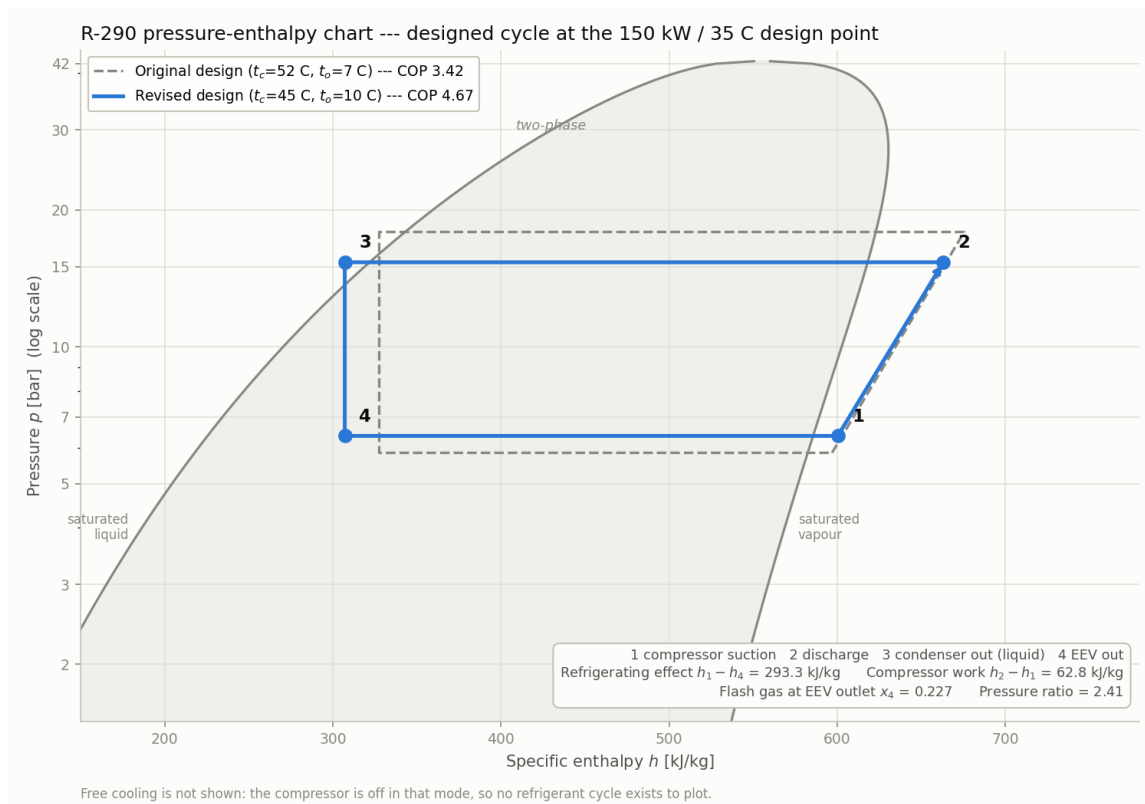
Figure 15.1. R-290 p-h chart of the designed cycle at the 150kW / 35 °C design point. The superseded original design is overlaid (dashed) for comparison.
