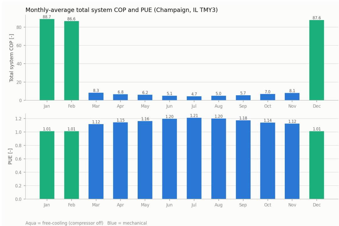
Figure 14.6. Monthly-average total-system COP and PUE. Aqua bars are free-cooling months (compressor off).
