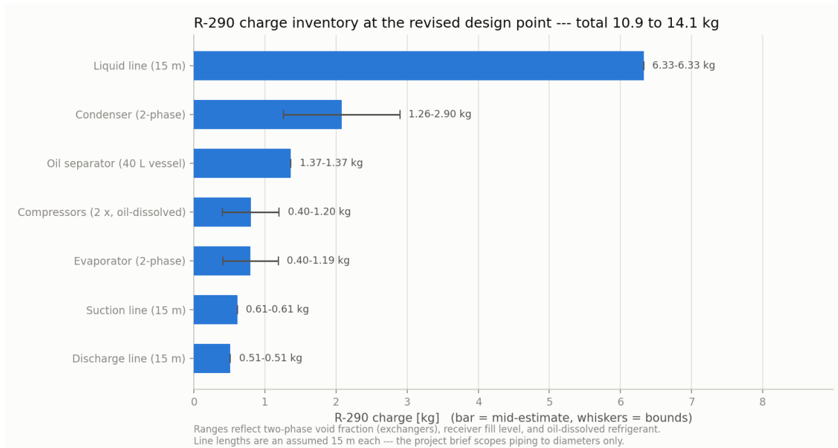
Figure 16.1. R-290 charge inventory at the revised design point. Whiskers show the bounds from void fraction, receiver fill level, and oil-dissolved refrigerant.
