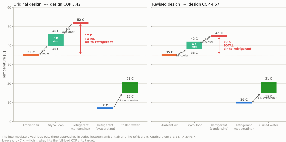
Figure 15.2. Temperature cascade from ambient air to chilled water, original vs. revised design. The condensing temperature is set by three approaches stacked in series.
