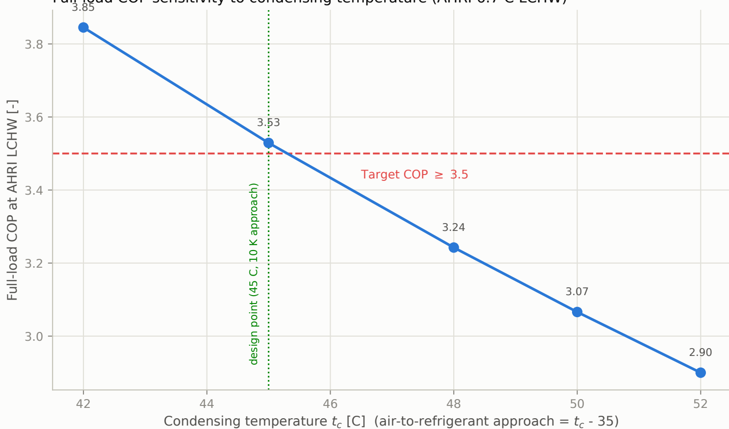
Full-load COP sensitivity to condensing temperature (AHRI 6.7 C LCHW)
