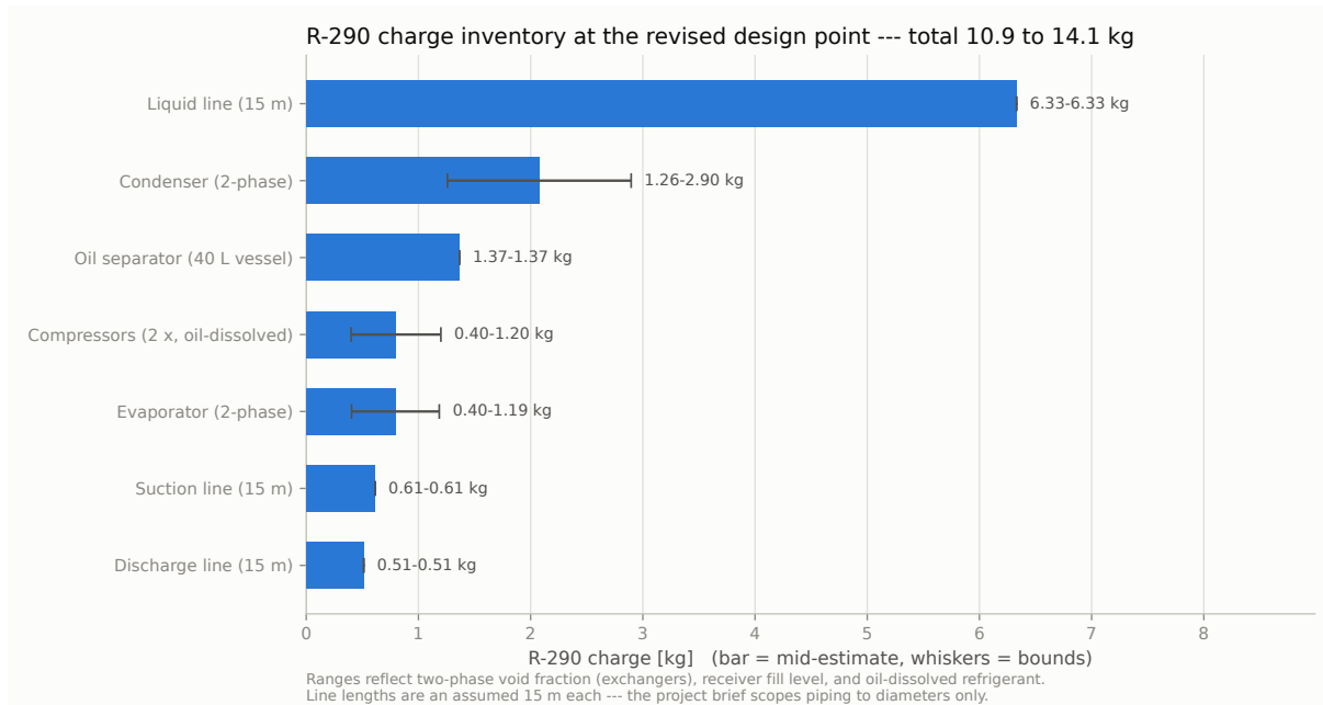
Figure 16.1. R-290 charge inventory at the design point. Whiskers show the bounds from void fraction, receiver fill level, and oil-dissolved refrigerant.
