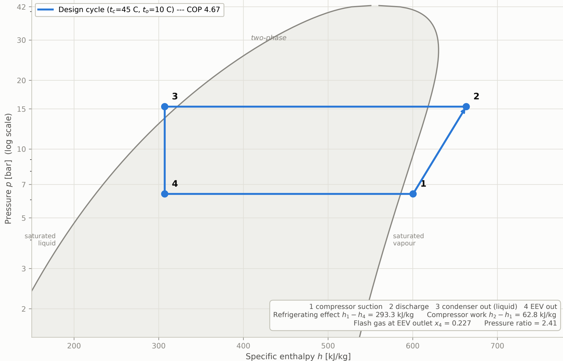
R-290 pressure-enthalpy chart --- designed cycle at the 150 kW / 35 C design point
