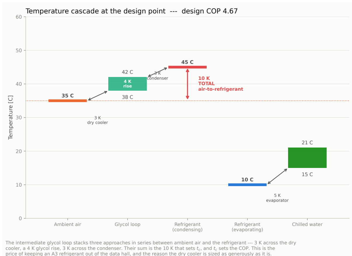
Figure 15.2. Temperature cascade from ambient air to chilled water at the design point. The condensing temperature is set by three approaches stacked in series.
