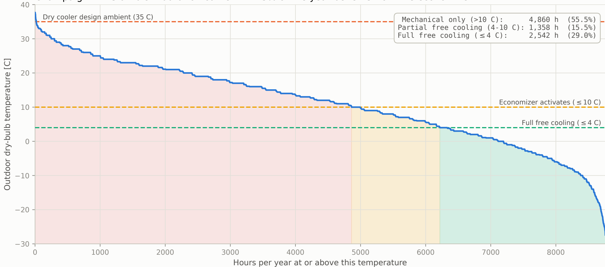
Champaign TMY3 ambient duration curve --- 44.5% of the year benefits from the economizer
