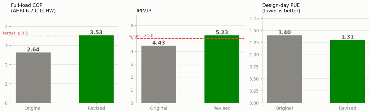
Figure 14.9. The revision's headline result: both required metrics move from failing to compliant, and the design-day PUE improves as a by-product.
