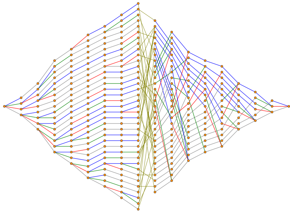
pyridine, STO-3G, (8e,8o): 16 qubits, K = 2765 terms (showing 40)
