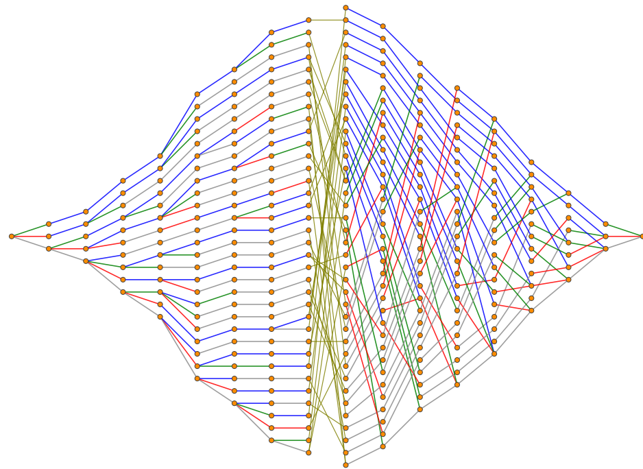
\text{BH}_3 , STO-6G: 16 qubits, K = 5437 terms (showing 40)
