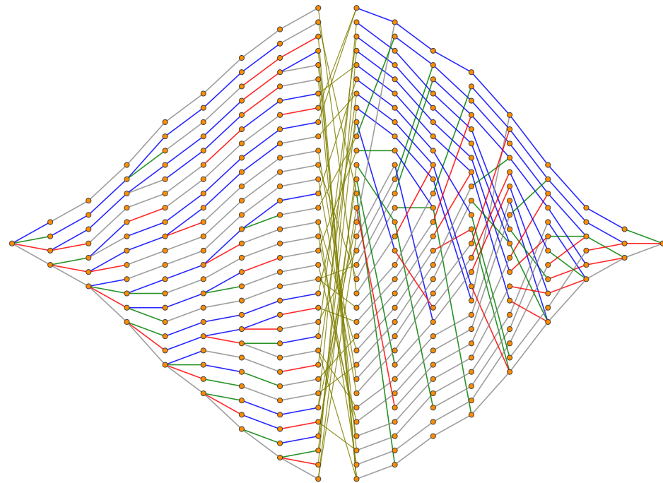
\text{BH}_3 , STO-3G: 16 qubits, K = 4201 terms (showing 40)
