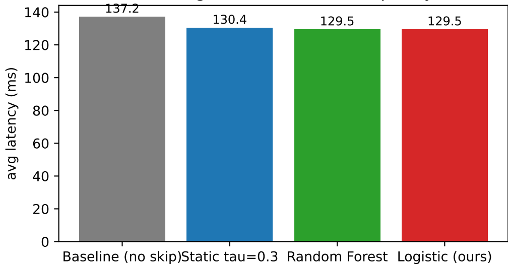
Cascade variants on ImageNet-V2 Matched-Frequency (A-IDK test)
