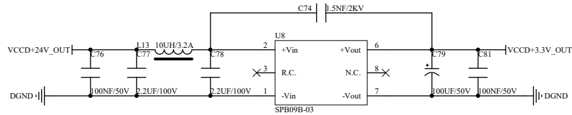
DC/DC+3.3V转换
