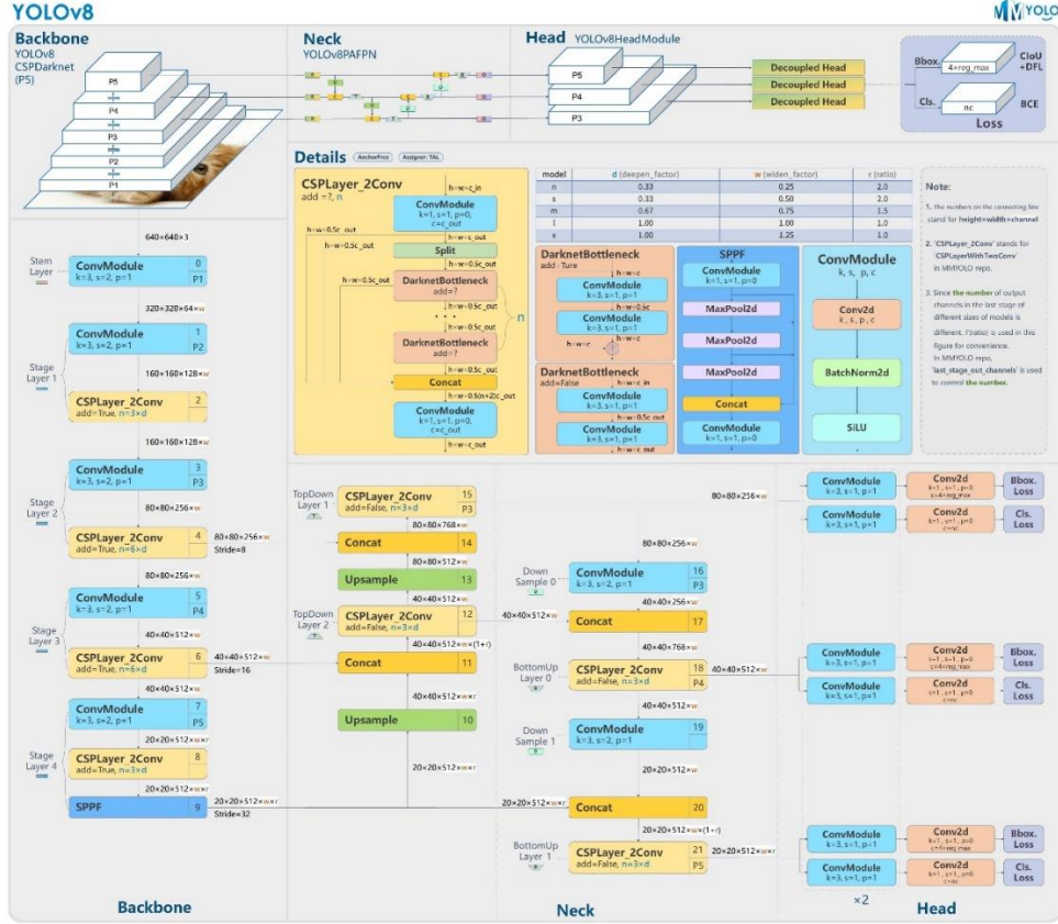
Figure 1. YOLO v8 network structure
