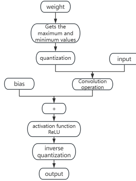
Figure 3. Quantization process
