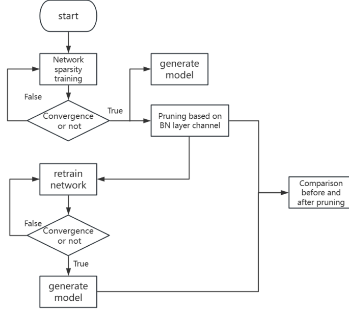
Figure 2. Pruning process
