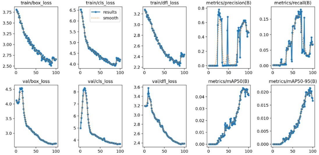
Figure 7. Training results of Yolo v8n network after pruning
