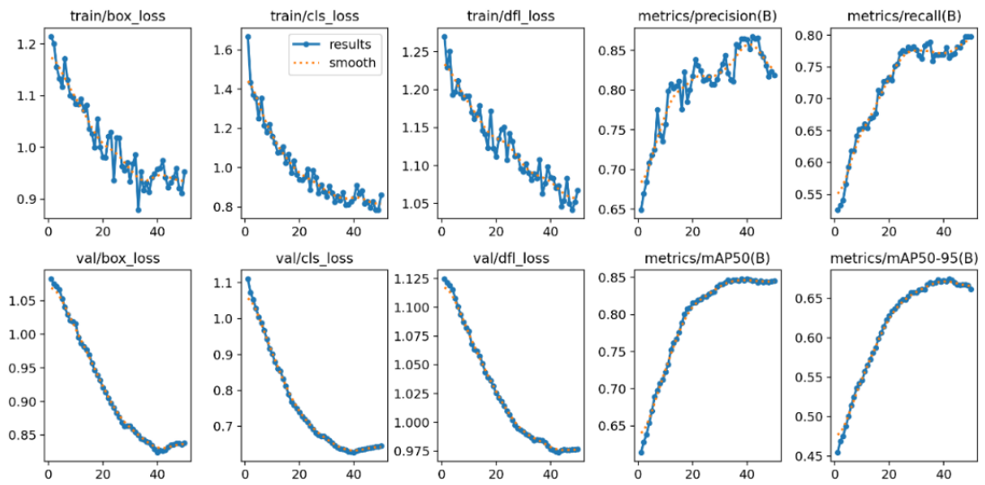
Figure 6. Training results of Yolo v8n network before pruning
