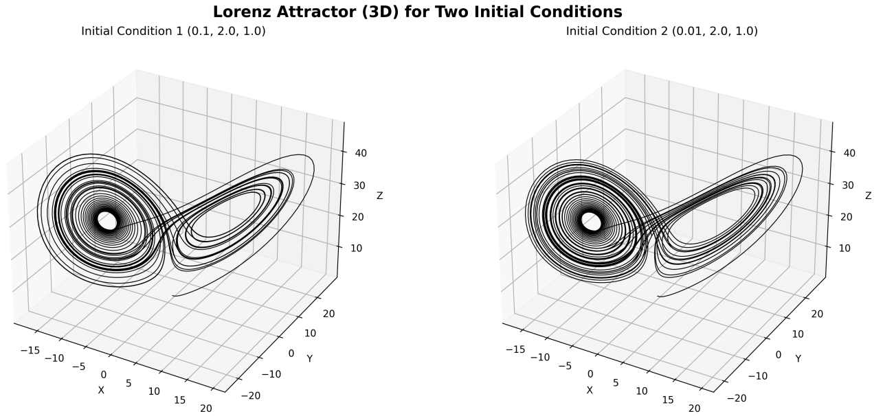
Figure 9: Comparison between two similar initial conditions of (0.01, 2.0, 1.0) and (0.1, 2.0, 1.0) and the time steps of \Delta t = 0.0073 to show the chaotic behavior of the system.
