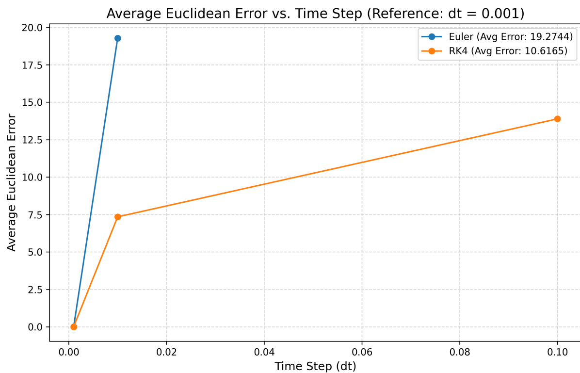
Figure 2: Lorenz attractor error analysis with initial state (1.0,1.0,1.0) and time step (0.001, 0.01, 0.1), and total simulation time of 40 seconds, For \Delta t > 0.01 , the solution is not stable enough to reliably reproduce the attractor shape.
