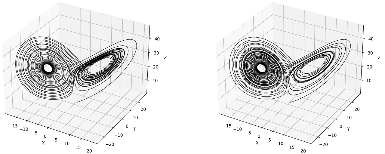
Figure 11: Comparison between two similar initial conditions of (1.0, 1.0, 1.0) and (1.0001, 1.0, 1.0) and the time steps of \Delta t = 0.0073 to show the chaotic behavior of the system.
