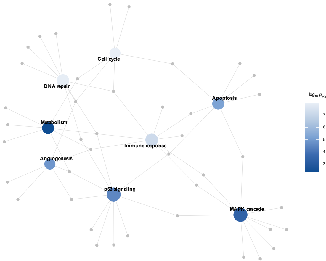
Pathway-gene enrichment network (synthetic demo)
