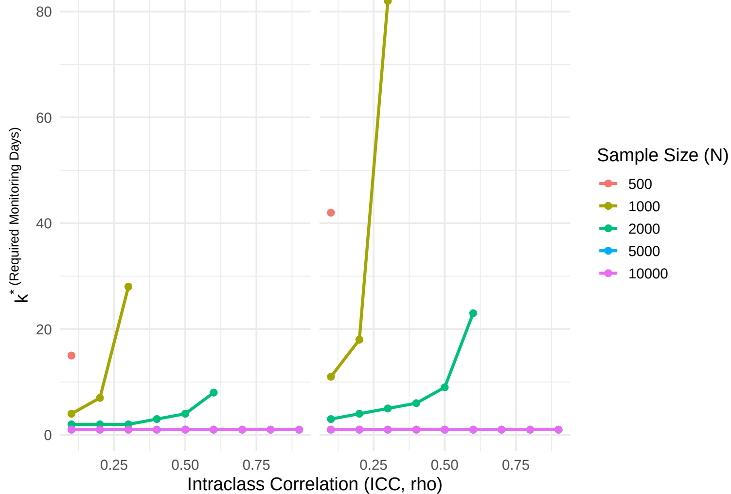
Conditional independence ( \phi = 0 )
