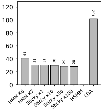
Holdout perplexity ( \downarrow )
