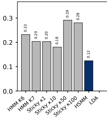
Duration KL ( \downarrow )
