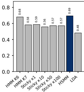
Reinit ARI ( \uparrow )
