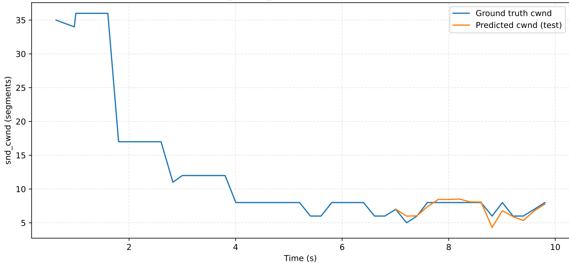
Trace trace_2 - snd_cwnd ground truth vs prediction
