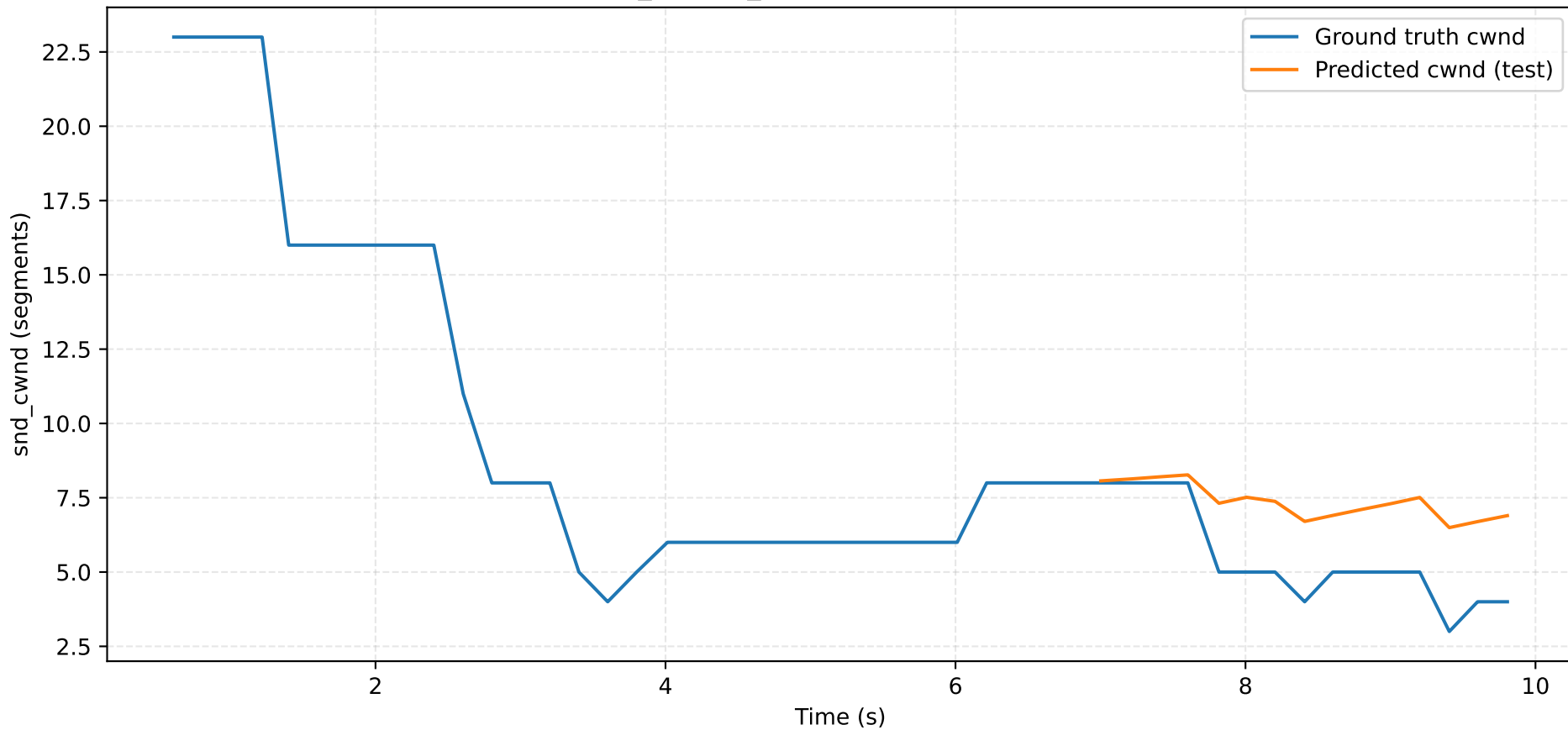
Trace trace_1 - snd_cwnd ground truth vs prediction
