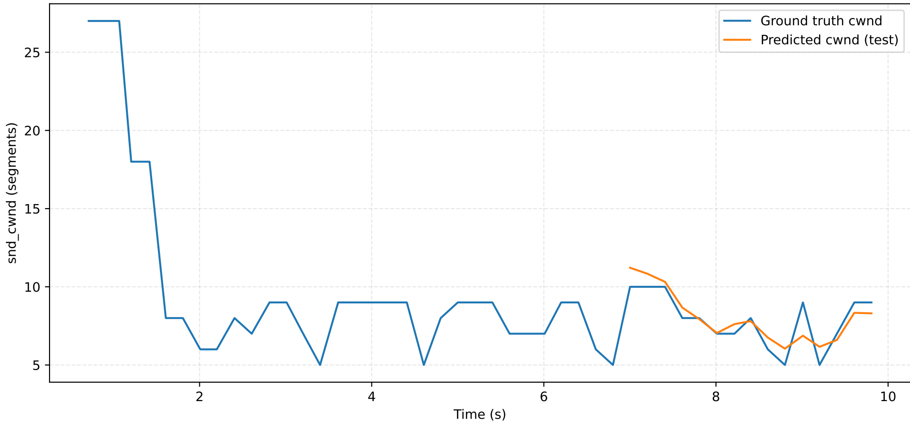
Trace trace_4 - snd_cwnd ground truth vs prediction
